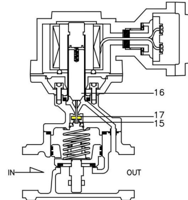
Normally Open
